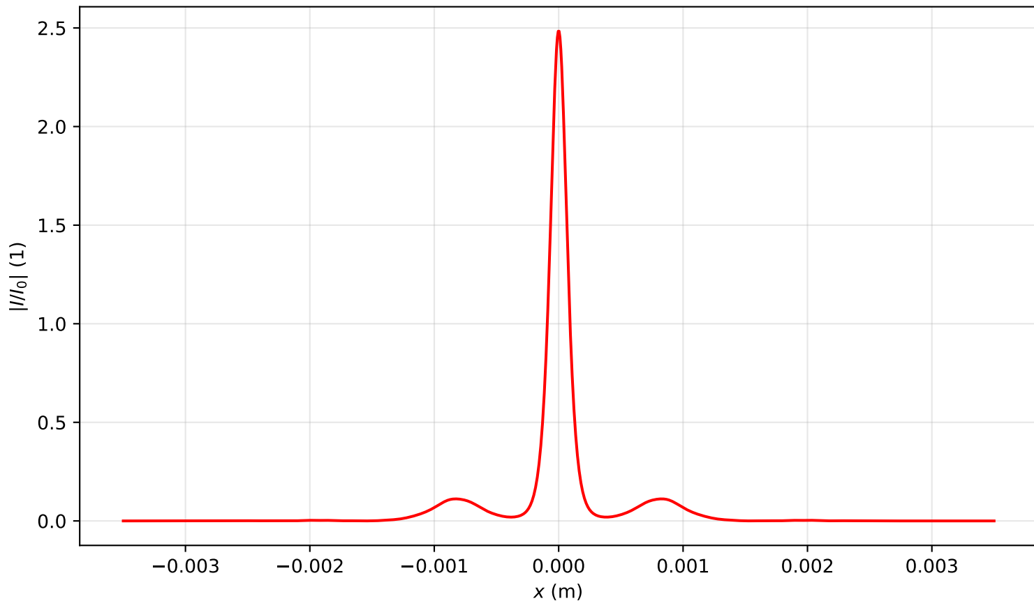
Intensity profile I(x, y = 0, z = 1.911)/I_0 , P_{in}=8.0P_{cr} , artificial time
